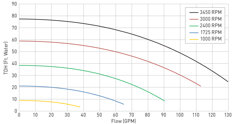
TRISTAR VS 950 PERFORMANCE COMPARISON
