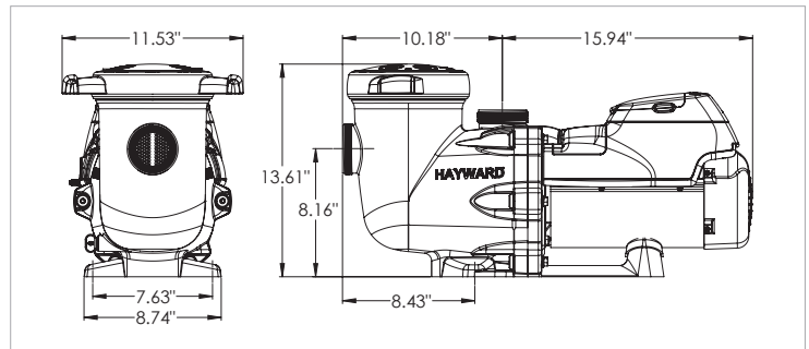
TRISTAR VS 950 DIMENSIONS (INCHES)
